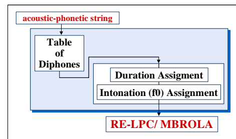
Figure 3: Prosodic module for Italian FESTIVAL followed by the synthesis engine module (RE_LPC and MBROLA)
