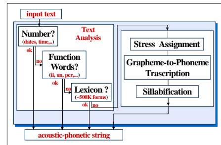
Figure 2: Text/Linguistic module for Italian FESTIVAL.
